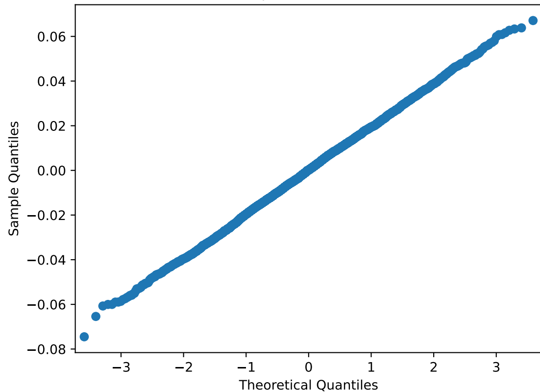
QQ-plot of residuals
