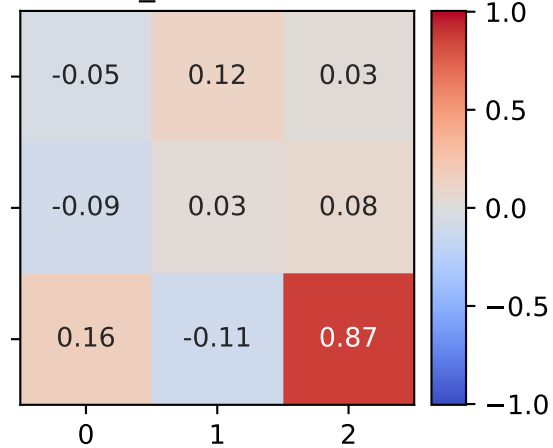
core_tensor[2, :, :]
