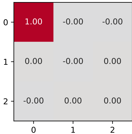
core_tensor[0, :, :]
